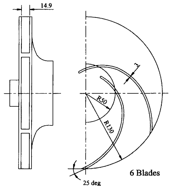
Fig. 2 Impeller geometry
