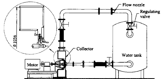
Fig. 1 Schematic view of the test rig
